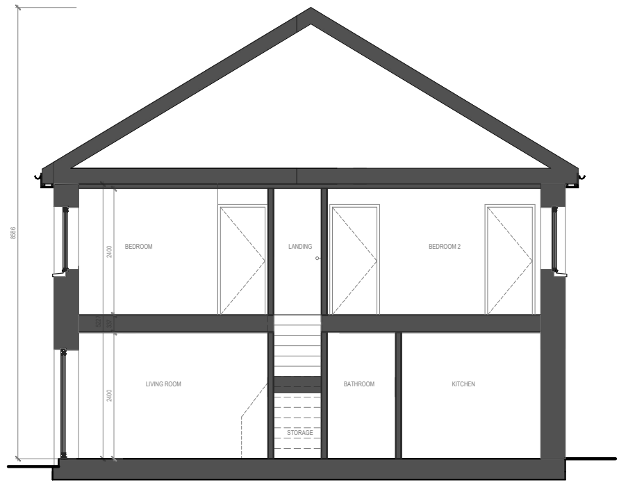
SECTION AA 2 BEDROOM ALTERNATIVE
